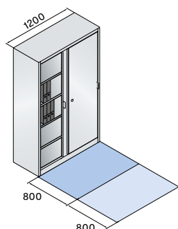
Sliding-door cabinet
