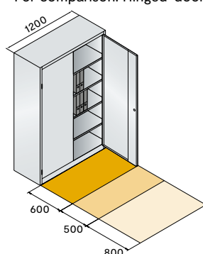
For comparison: Hinged-door cabinet
