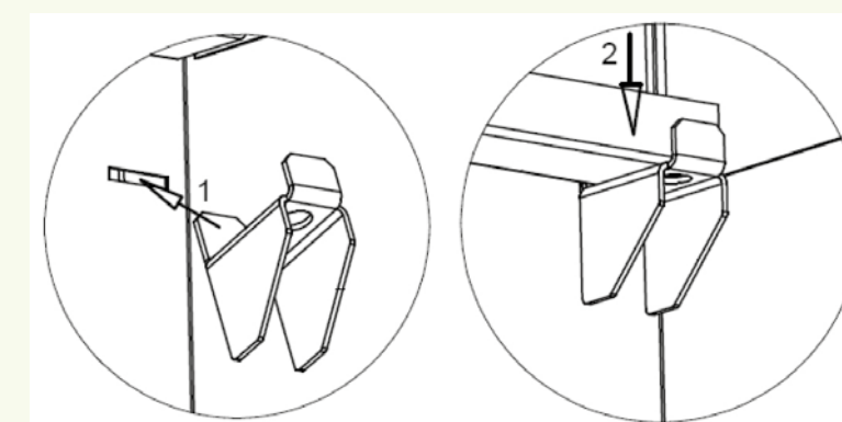
Riulitoe paigaldamine
